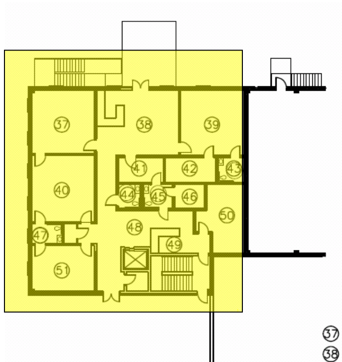
BASEMENT NEW ADDITION FLOOR PLAN SCALE: NTS
